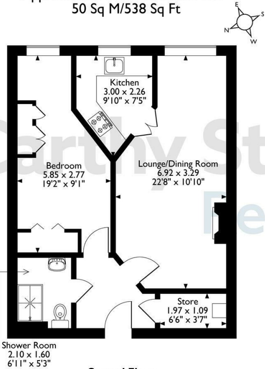
Second Floor The position & size of doors, windows, appliances and other features are approximate only. © ehouse. Unauthorised reproduction prohibited. Drawing ref. dig/8660513/DST.
